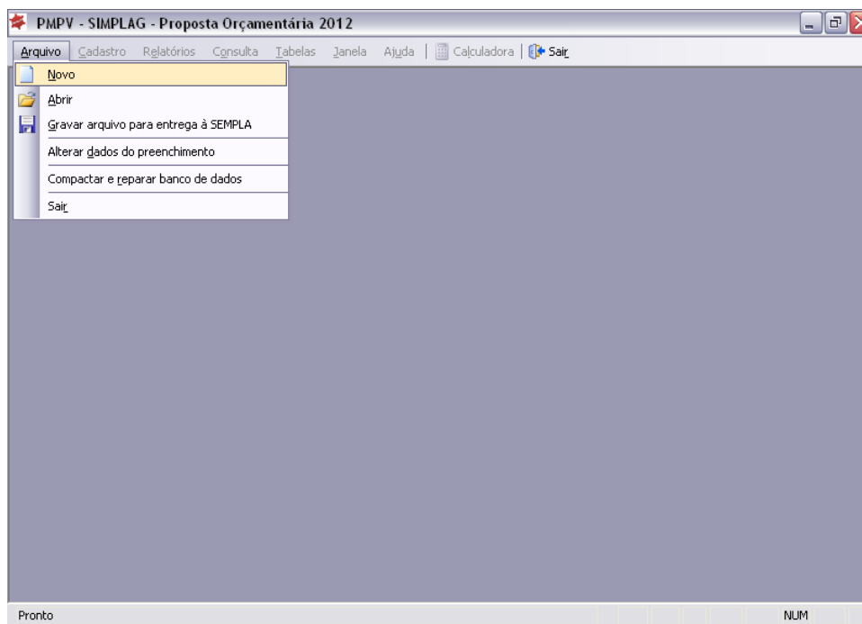
Figura 1 – Tela Principal
